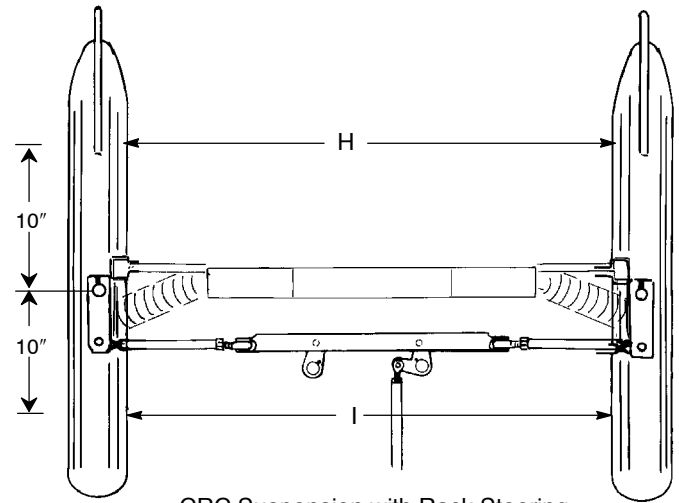
CRC Suspension with Rack Steering
